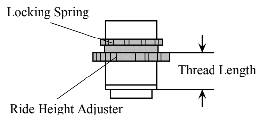
[Rear Ride Height Adjuster Assy]
