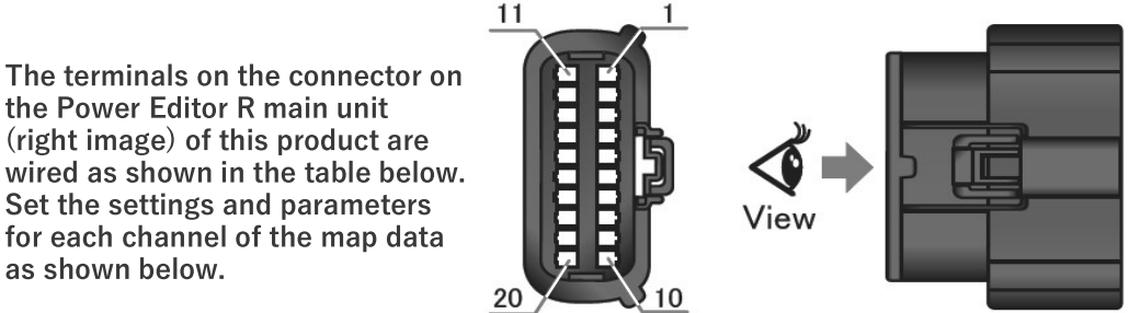
Power Editor R main unit connector
